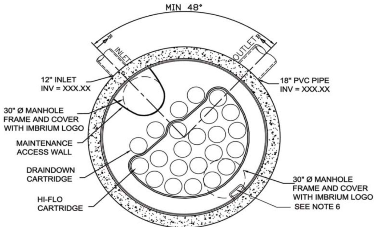
JELLYFISH CROSS SECTION A-A
